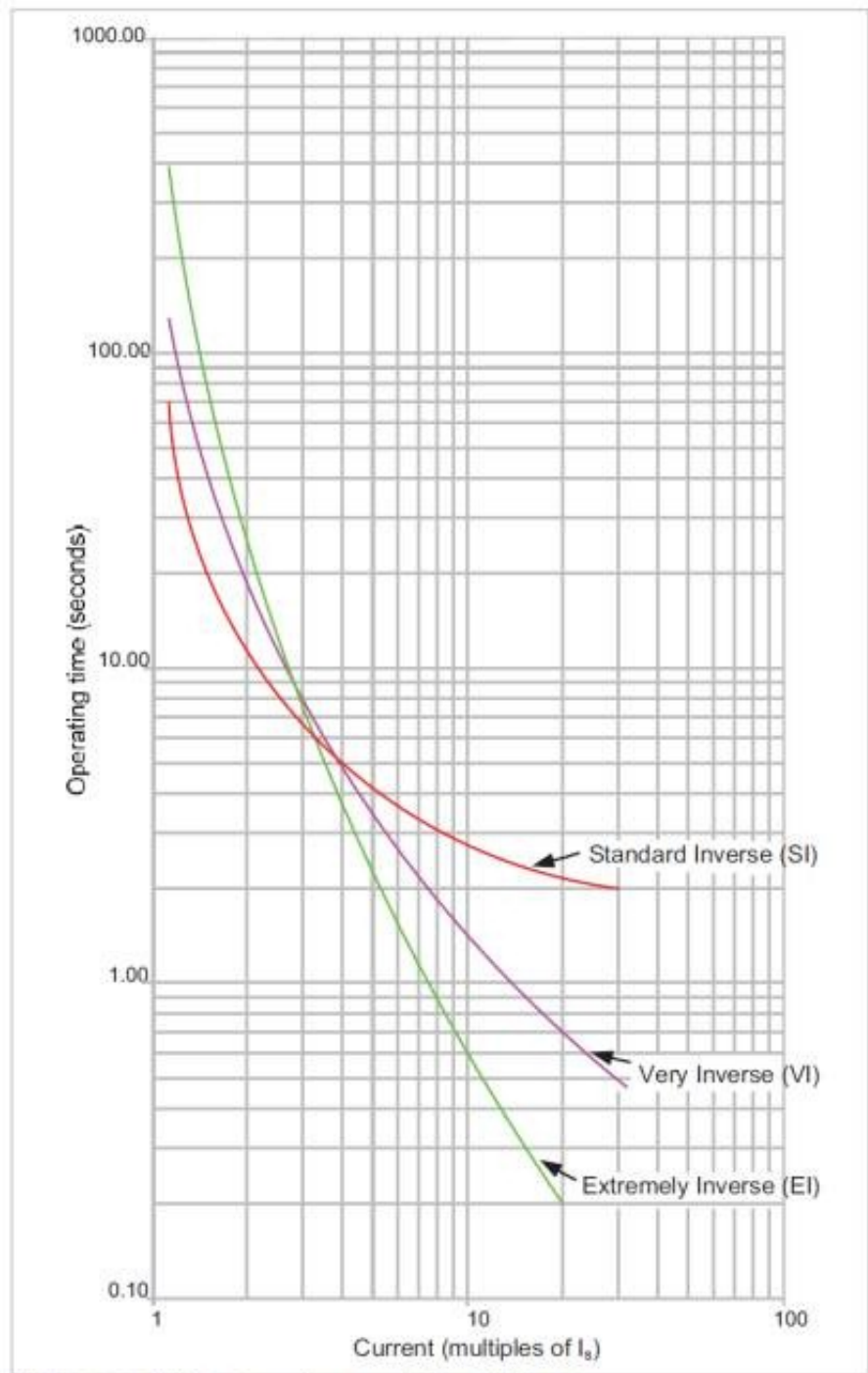
IEC 60255 IDMT relay characteristics; TMS=1.0
